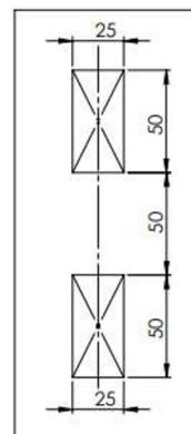
PANEL CUTOUT
